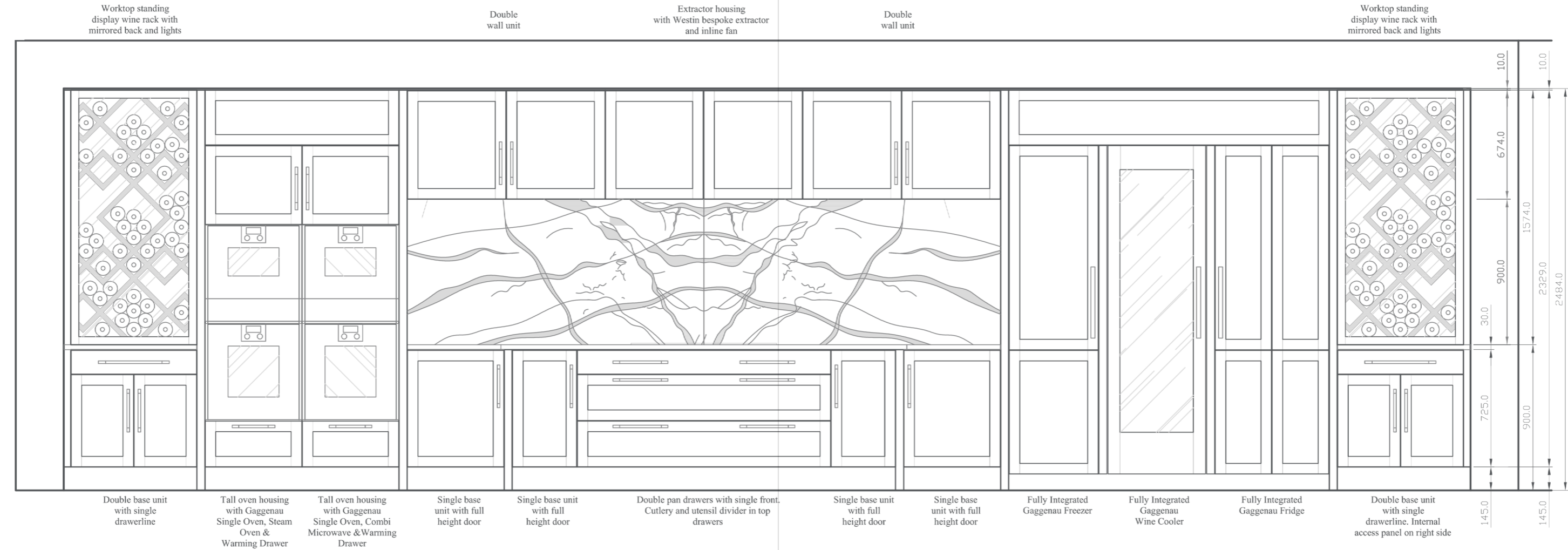
PLAN ELEVATION
